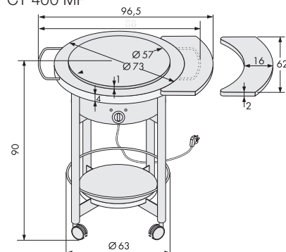
TeppanMobil CT 400 MP
