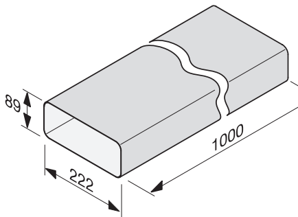
Canal plat 1000 mm DFK-R 1000 ①
