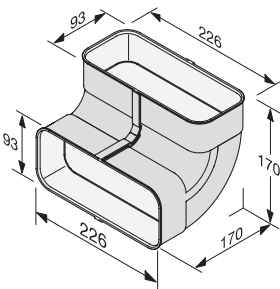
Courbe verticale 90° 170 mm DFK-BV 90 ②
